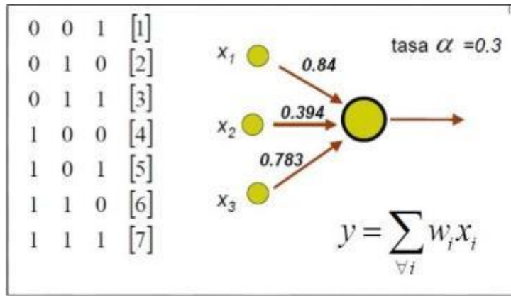
Figura 8.Red Adaline
