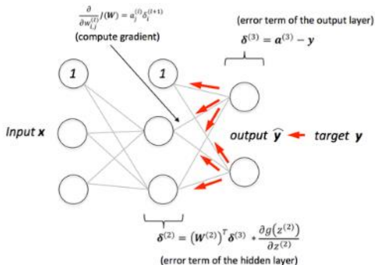
Figura 9.Backpropagation
