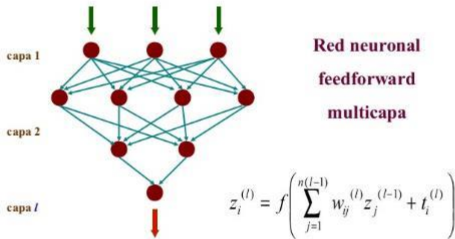
Figura 5. Red Feedforward
