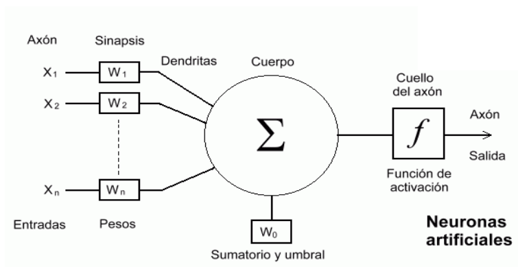
Figura 2. Neurona Artificial
